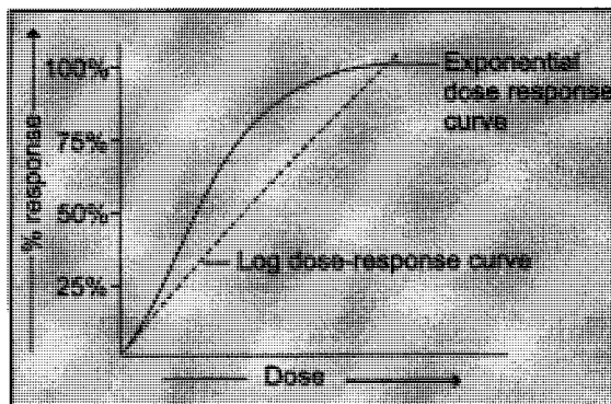
Fig. 1.5.4: Hyperbolic or exponential dose-response curve.
